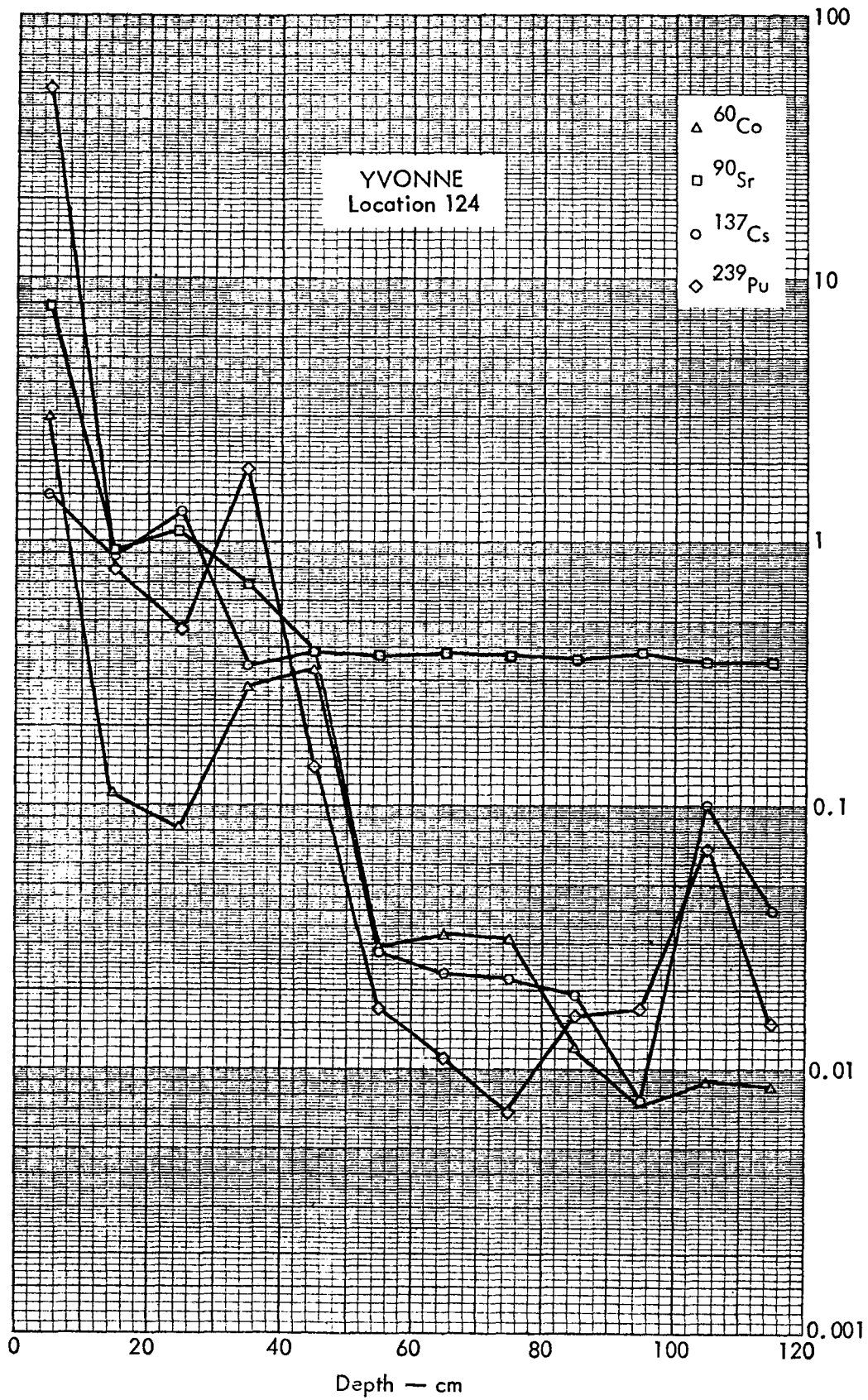
FIGURE 103. ACTIVITIES OF SELECTED RADIONUCLIDES AS A FUNCTION OF SOIL DEPTH
